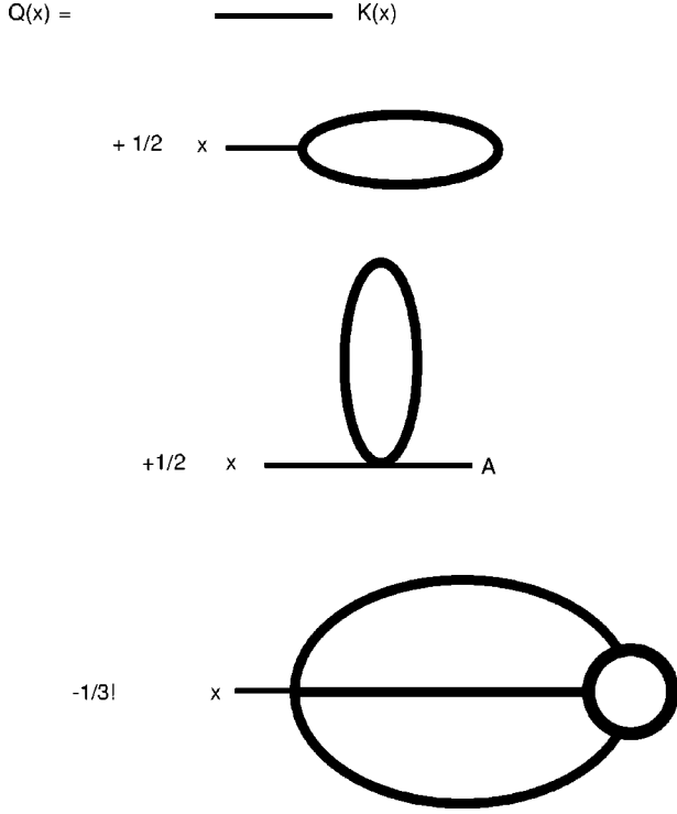
FIG. 1. Diagrammatic representation of the functional DS equation for the quantum effective drift force Q(A) in the presence of external sources A , Eq. (6.1). The vertices are the tree-level vertices of the drift force K . The internal lines represent the exact gluon propagator D(A) in the presence of the external source. The circle is the exact three-gluon vertex of the quantum effective action \Gamma(A) in the presence of the external source.
