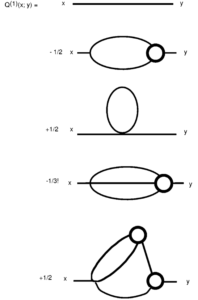
FIG. 2. Diagrammatic representation of the DS equation for the gluon propagator, Eq. (8.1). The vertices are the tree level vertices of the drift force K . The internal lines are the exact gluon propagator D with sources set to 0. The circles represent the exact three- and four-gluon vertices of the quantum effective action \Gamma , with sources set to 0.
